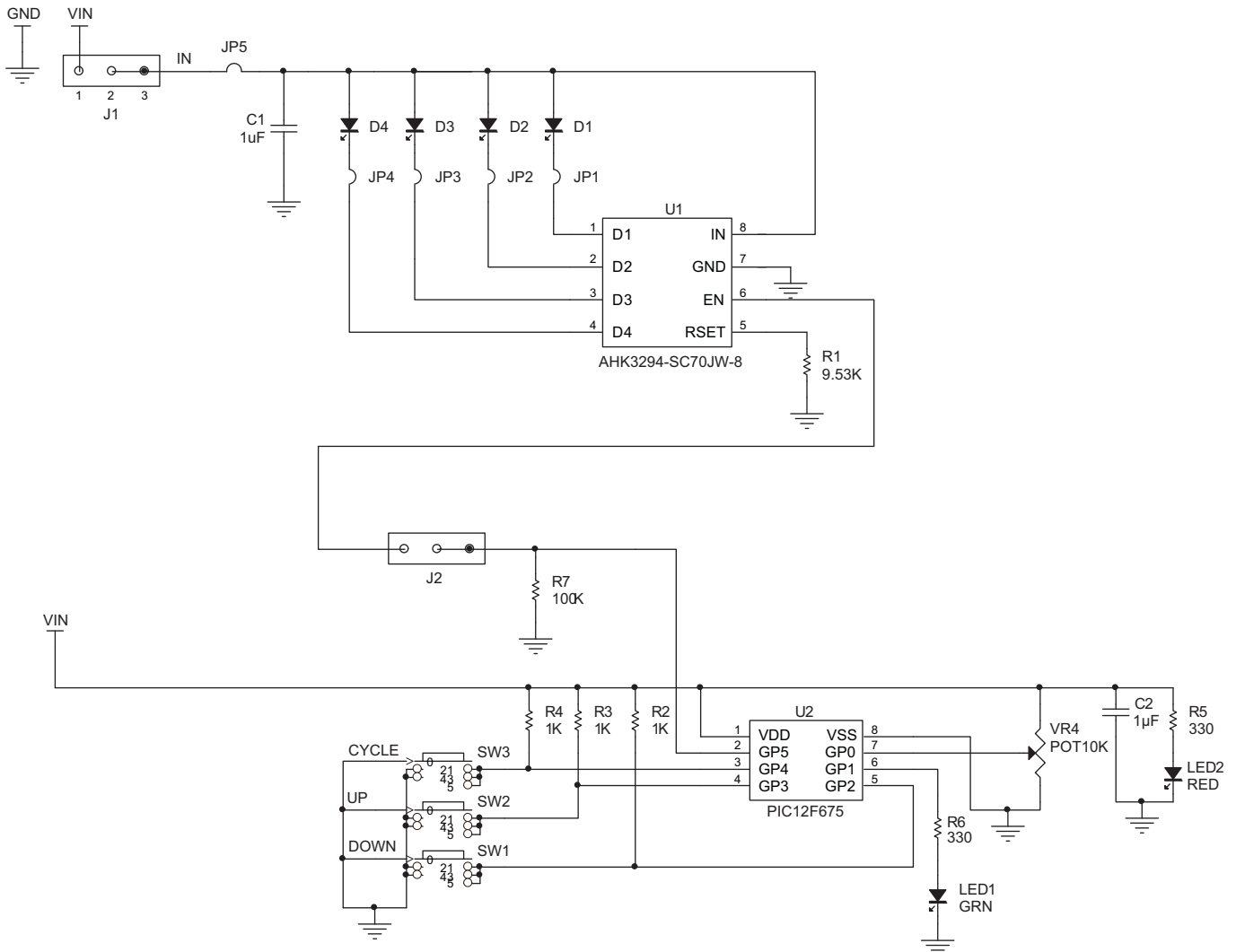
Figure 4: AHK3294 Evaluation Board Schematic.
